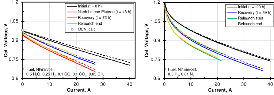
Figure 3: Left: I-V-curves of Stack N on syngas at indicated instants. Right: I-V-curves on H 2 /N 2 mixture at indicated instants. Solid lines represent voltage of lower cell. T_{\text{stack}} = 700^{\circ}\text{C} . Noisy data were fitted with a hyperbolic plus linear term for better visibility.
