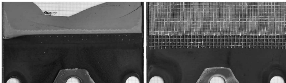
Figure 7: Photos of one layer of Stack P after the tests with phenol. Left: surface of the anode substrate. Right: nickel meshes for contacting.
