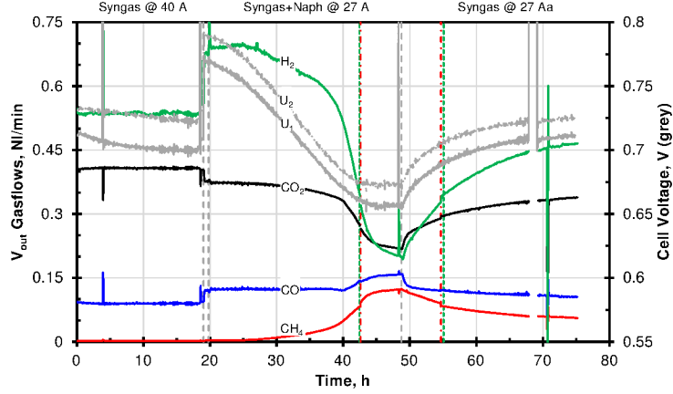
Figure 4: Flow rate of main gas components CO, CO 2 , CH 4 and H 2 in the anode exhaust gas during measurement at Stack N. U_1 voltage of lower cell and U_2 voltage of upper cell. T_{\text{stack}} = 700^\circ\text{C} .
