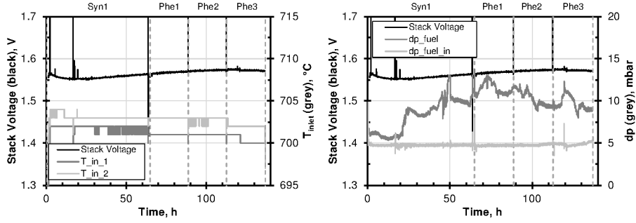
Figure 5: Left: Trends of stack voltage and inlet temperature of lower cell ( T_{in,1} ) and upper cell ( T_{in,2} ) of Stack P. Right: Pressure drop on fuel gas side ( p_{fuel} ) and overpressure at fuel inlet ( p_{fuel,in} ) of Stack P.
