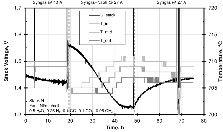
Figure 2: Course of stack voltage and temperatures of the upper cell (inlet, middle, outlet). Syngas as main gas, naphthalene concentration 2 \text{ g/Nm}^3 .
