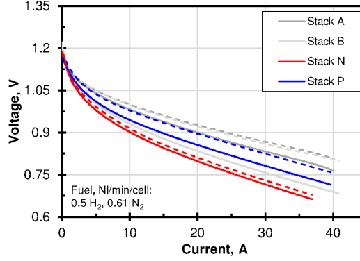
Figure 1: Initial I-V-curves at 0.5 Nl/min/cell H_2 and 0.61 Nl/min/cell N_2 of Stack N and P compared to previously tested stacks. Solid line lower layer (Cell 1), dashed line upper layer (Cell# \geq 2 ). T_{\text{stack}} = 700^\circ\text{C} . Due to high noise data from Stack P was fitted with a hyperbolic plus linear term for better visibility.
