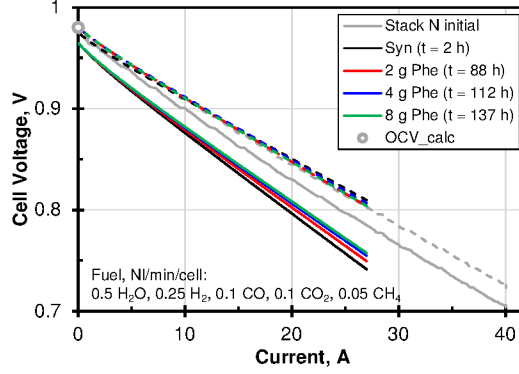
Figure 6: I-V-curves of Stack P on syngas plus 0, 2, 4 and 8 g/Nm 3 of phenol together with data from Stack N. T_{\text{stack}} = 700^{\circ}\text{C} . Data for Stack P was fitted with a hyperbolic plus linear term for better visibility.
