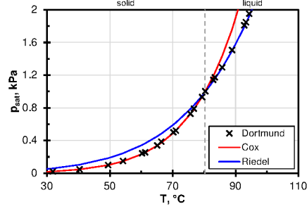
Figure .8: Trend of saturation pressure of naphthalene calculated with Cox and Riedel equation. Experimental reference values are found in [35].
